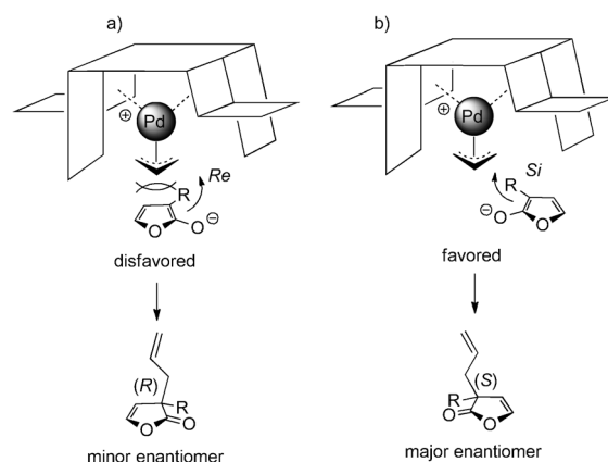
Figure 1. Model for the explanation of the selectivity.
