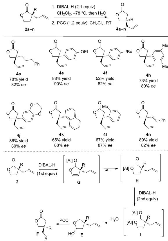
Scheme 4. Asymmetric synthesis of \beta -quaternary butyrolactones. All reactions were run on a 0.25 mmol scale. Yield is that of product isolated after two steps. Enantiomeric excess was determined by SFC analysis using a chiral stationary phase.
