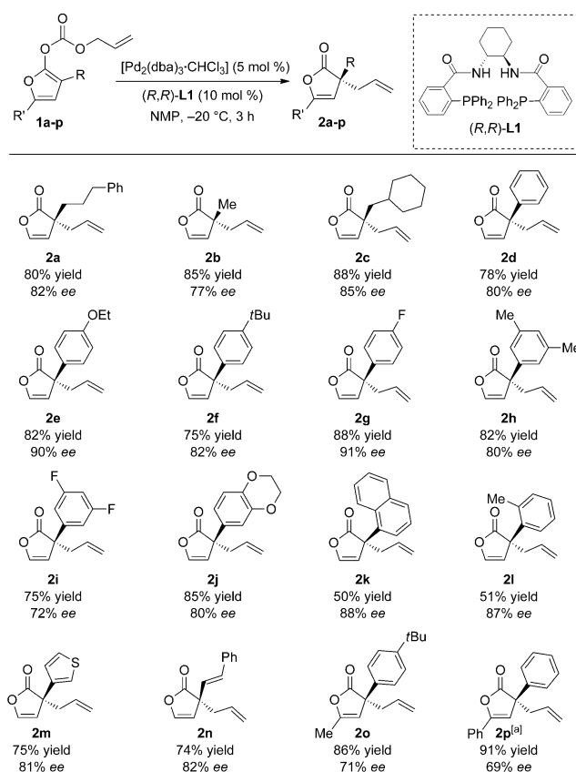
Scheme 2. Scope of the palladium-catalyzed allylic alkylation of allyl dienol carbonates 1a–p . All reactions were run on a 0.25 mmol scale. Enantiomeric excess was determined by SFC analysis using a chiral stationary phase. [a] Reaction run in CH 3 CN.
