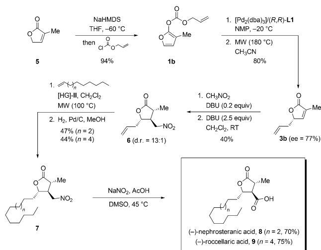
Scheme 5. Application of the palladium-catalyzed allylic alkylation to the synthesis of 8 and 9 . DBU = 1,8-diazabicyclo[5.4.0]undec-7-ene, DMSO = dimethylsulfoxide, [HG]-II = Hoveyda–Grubbs second generation catalyst, HMDS = hexamethyldisilazide.
