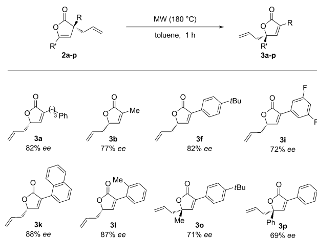
Scheme 3. Microwave-assisted Cope rearrangement of \alpha -quaternary butenolides: a straightforward access to \gamma -tertiary and \gamma -quaternary 2(5H)furanones. All reactions were run on a 0.2 mmol scale. Enantiomeric excess was determined by SFC analysis using a chiral stationary phase.
