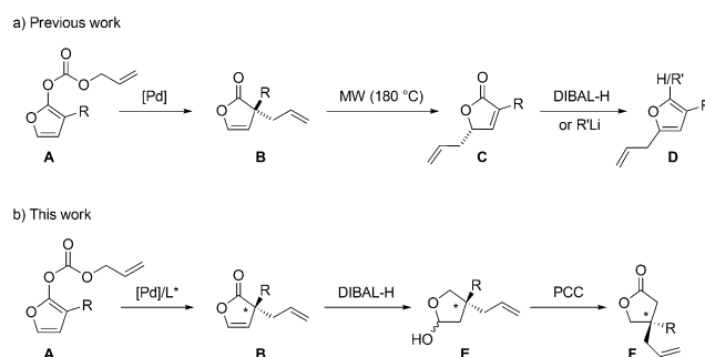
Scheme 1. a) One-pot, four-step, sequence for the synthesis of poly-substituted furans by Pd-AAA. b) Enantioselective synthesis of \alpha -quaternary butenolides and \beta -quaternary butyrolactones by Pd-AAA. DIBAL-H = diisobutylaluminum hydride, PCC = pyridinium chlorochromate, MW = microwave.
